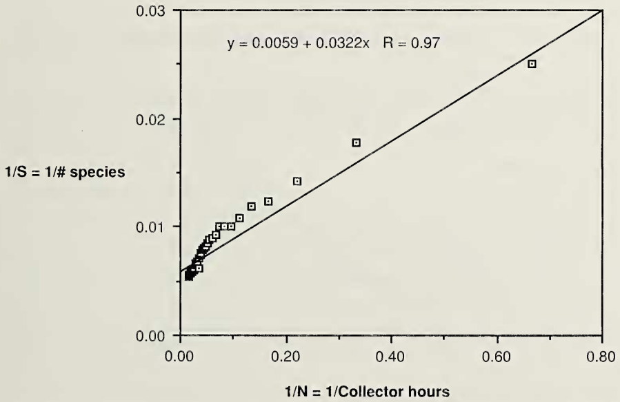
Figure 2b. Reciprocal Plots of species vs. collector-hours, Laguna Encantada, 1985.
